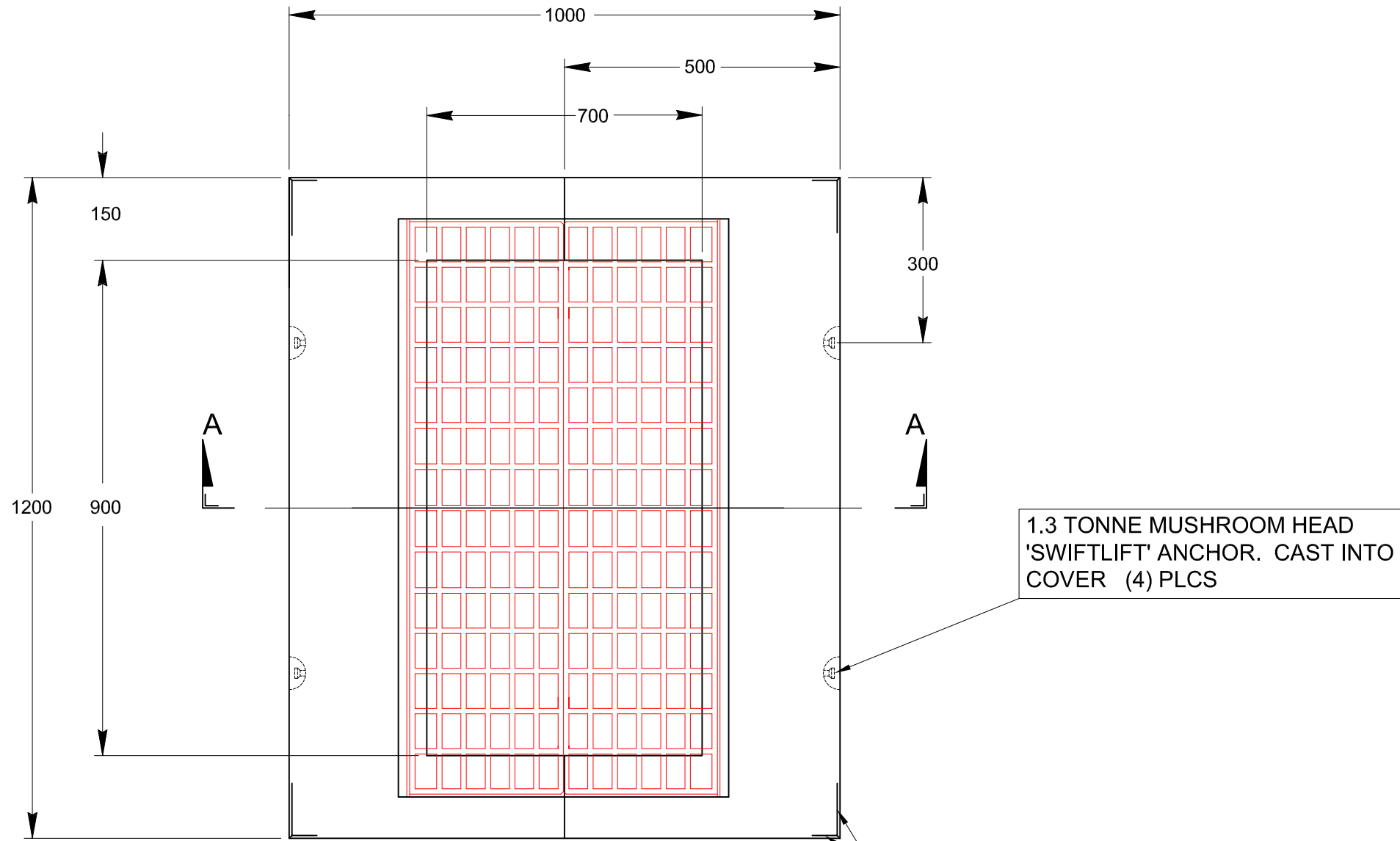
PLAN VIEW
