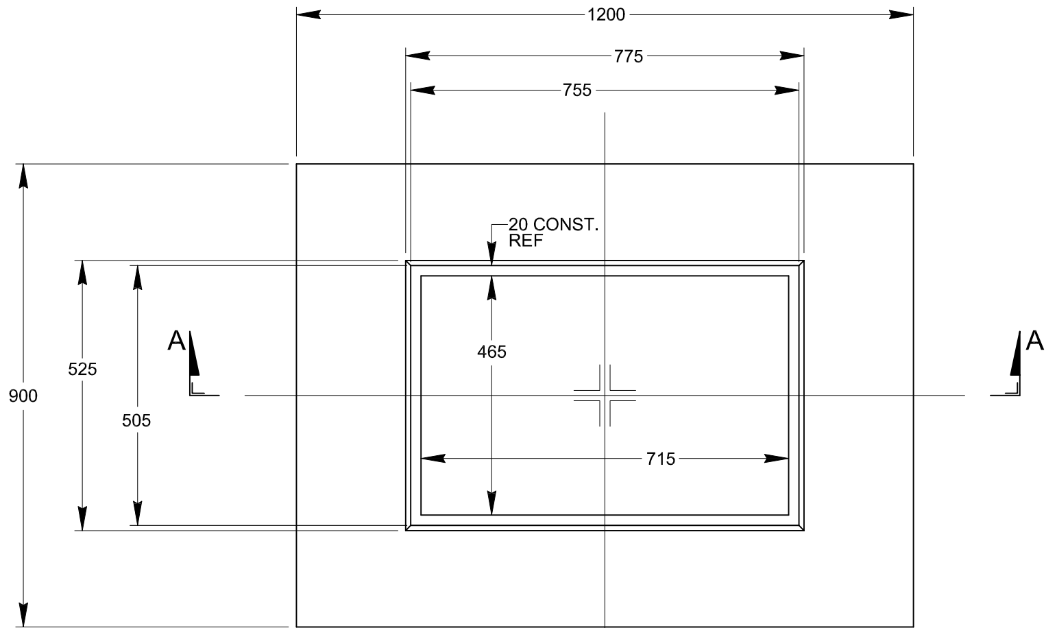
PLAN VIEW OF ACCESS COVER
