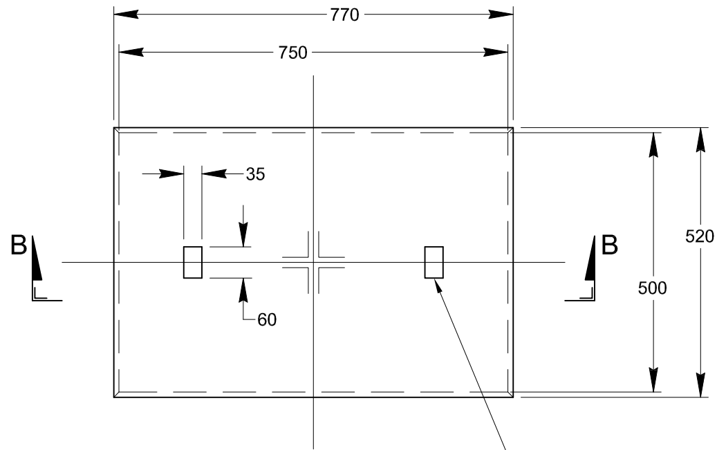
PLAN VIEW OF LID
